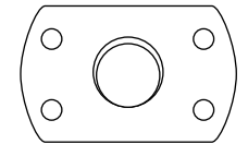
5/16-18 Tapping Plate, Qty - 16, Part Number 200.50
